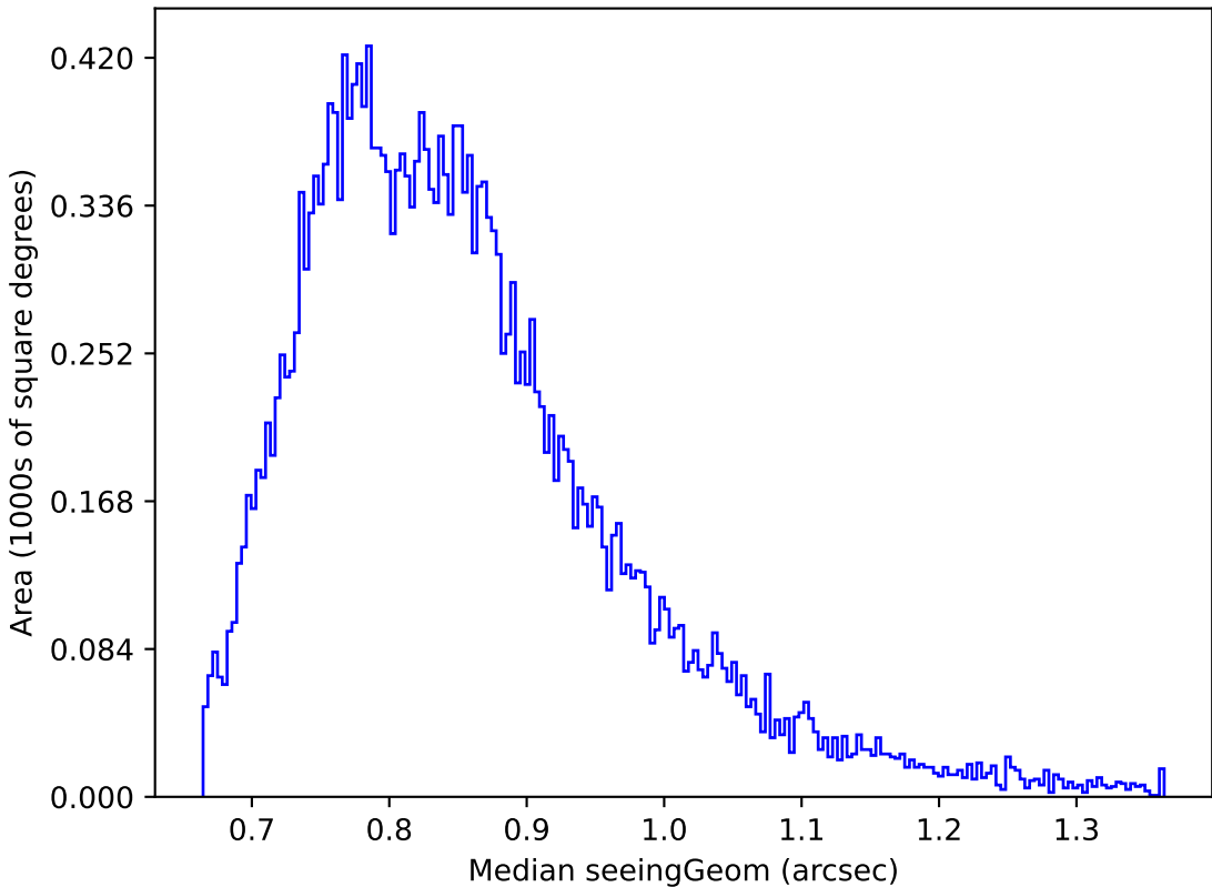
weather_cloudso6v3.4_10yrs Yr 1 z band: Median seeingGeom
