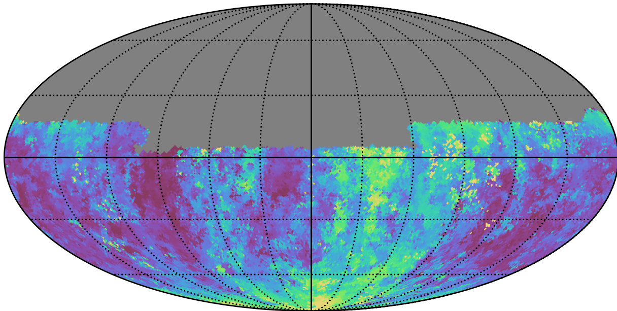
weather_cloudso6v3.4_10yrs Yr 1 u band: Median seeingGeom
