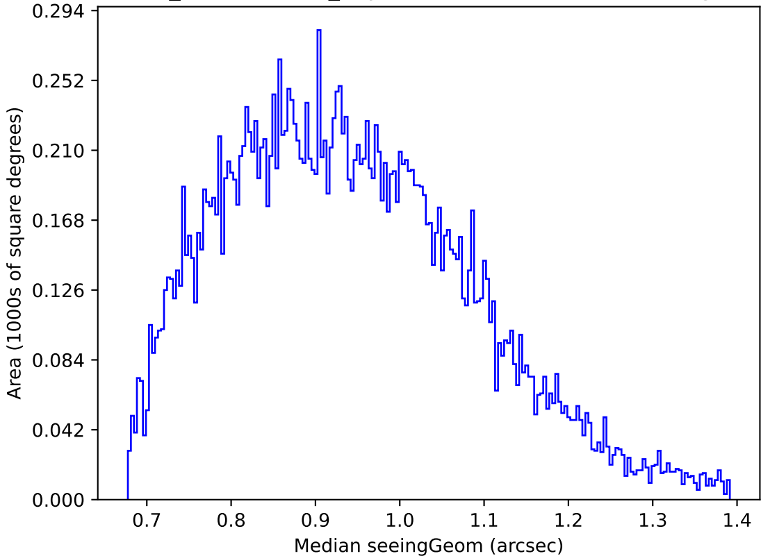
weather_cloudso6v3.4_10yrs Yr 1 u band: Median seeingGeom
