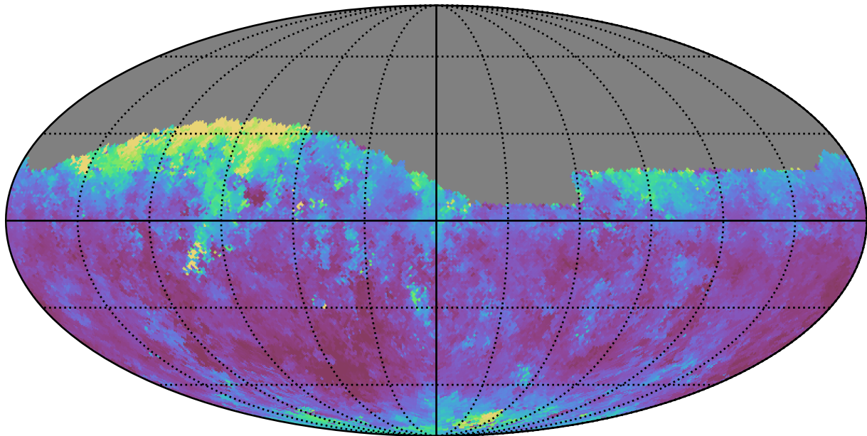
weather_cloudso6v3.4_10yrs Yr 1 i band: Median seeingGeom
