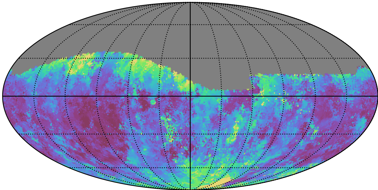
weather_cloudso6v3.4_10yrs Yr 1 g band: Median seeingGeom
