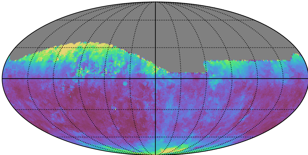
weather_cloudso6v3.4_10yrs Yr 1 all bands: Median seeingGeom
