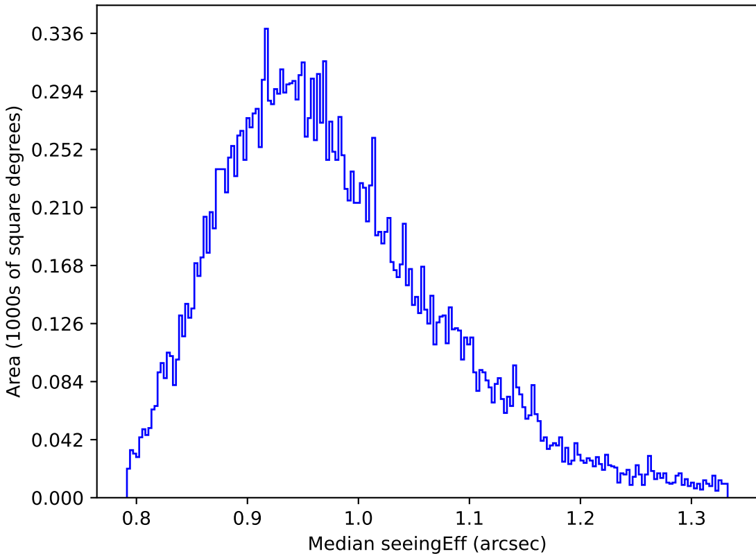
weather_cloudso6v3.4_10yrs Yr 1 y band: Median seeingEff
