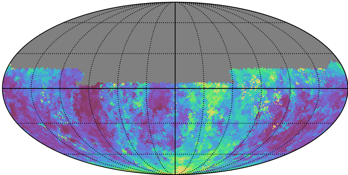
weather_cloudso6v3.4_10yrs Yr 1 u band: Median seeingEff
