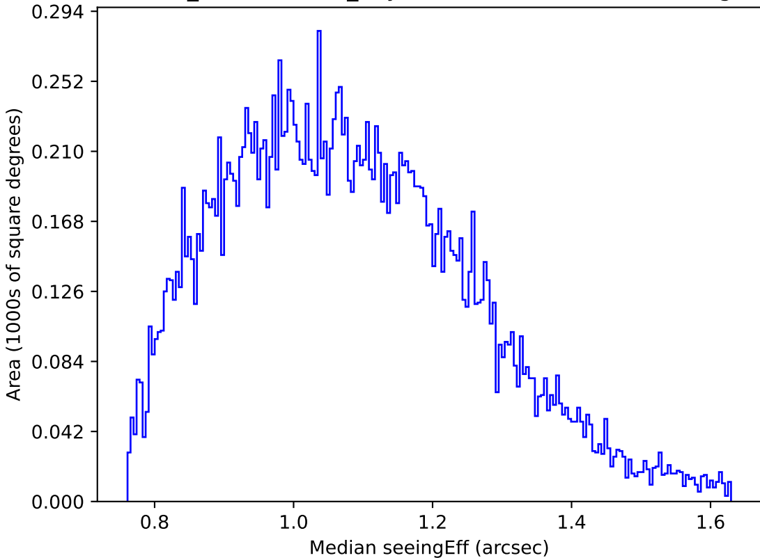
weather_cloudso6v3.4_10yrs Yr 1 u band: Median seeingEff
