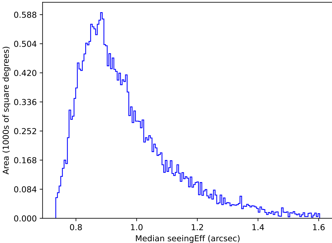
weather_cloudso6v3.4_10yrs Yr 1 r band: Median seeingEff
