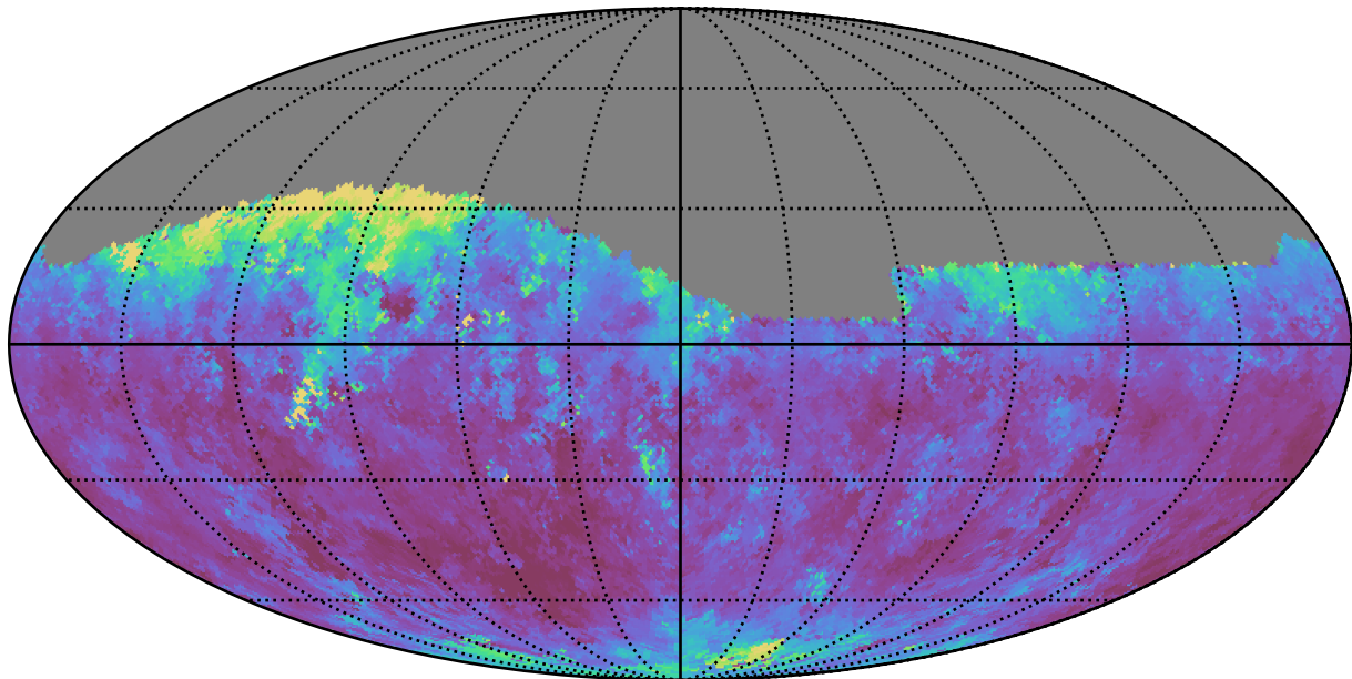
weather_cloudso6v3.4_10yrs Yr 1 i band: Median seeingEff
