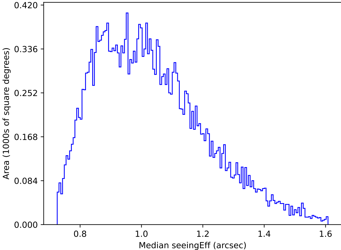
weather_cloudso6v3.4_10yrs Yr 1 g band: Median seeingEff
