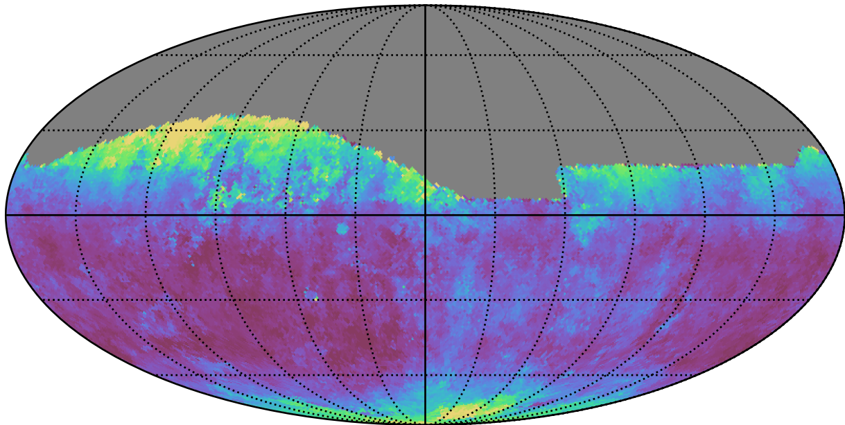
weather_cloudso6v3.4_10yrs Yr 1 all bands: Median seeingEff
