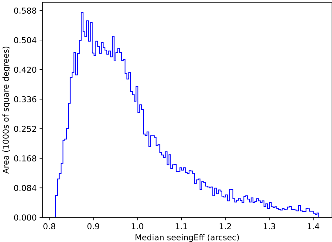
weather_cloudso6v3.4_10yrs Yr 1 all bands: Median seeingEff
