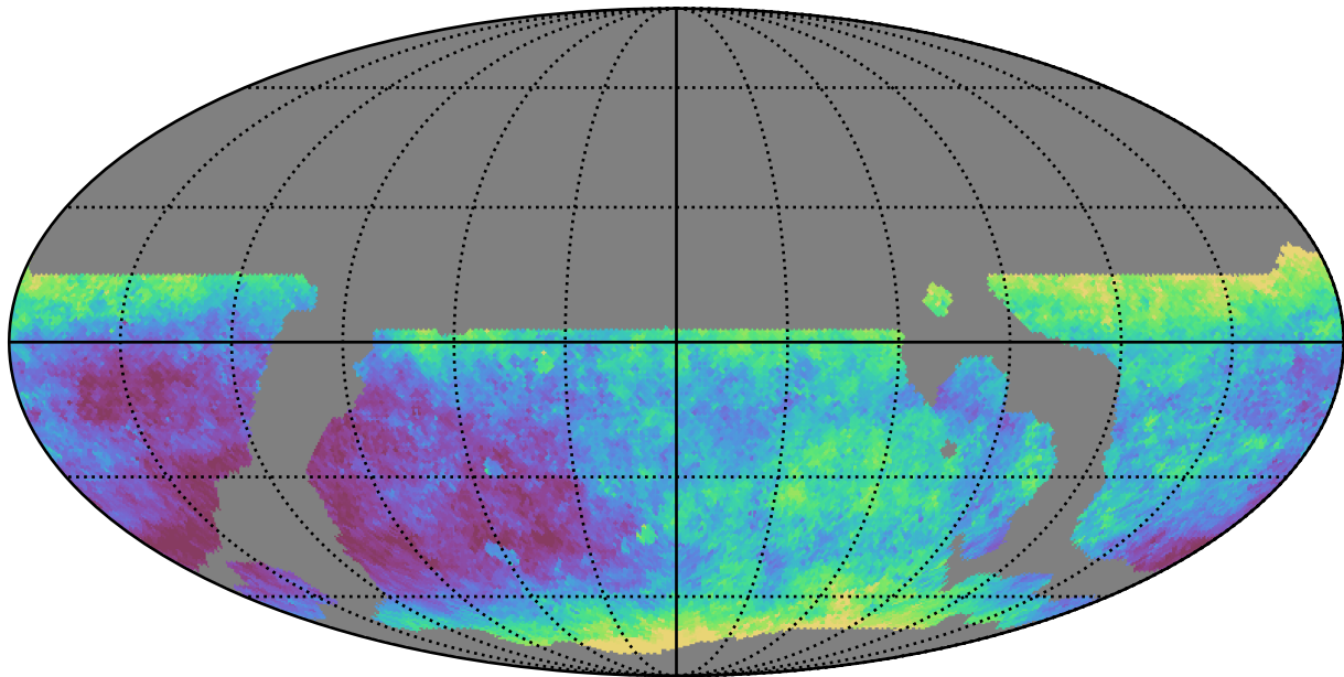
weather_cloudso6v3.4_10yrs WFD z band: Median seeingEff
