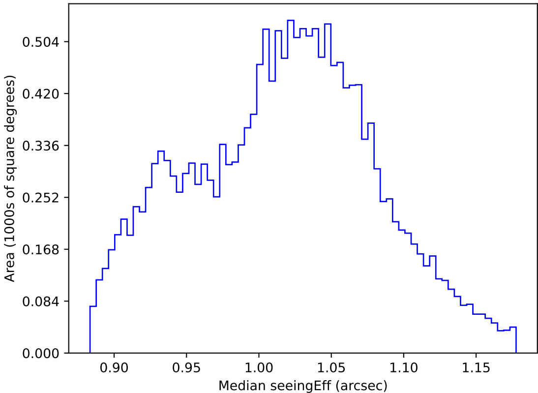
weather_cloudso6v3.4_10yrs WFD z band: Median seeingEff
