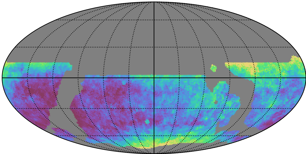
weather_cloudso6v3.4_10yrs WFD y band: Median seeingEff
