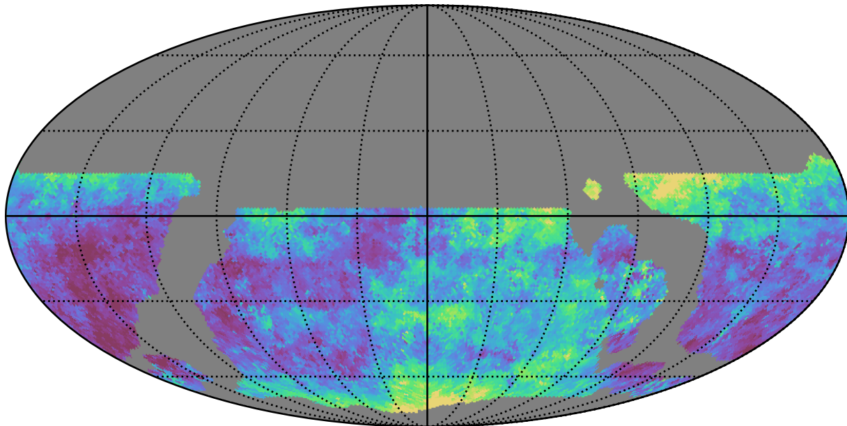
weather_cloudso6v3.4_10yrs WFD u band: Median seeingEff
