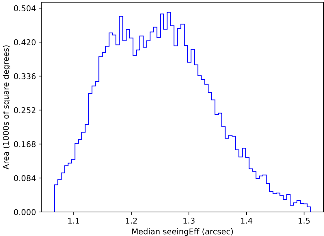
weather_cloudso6v3.4_10yrs WFD u band: Median seeingEff
