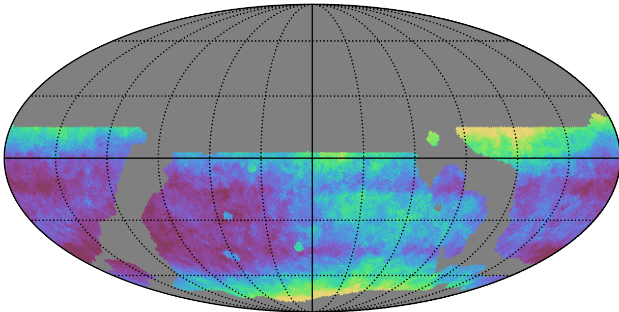
weather_cloudso6v3.4_10yrs WFD r band: Median seeingEff
