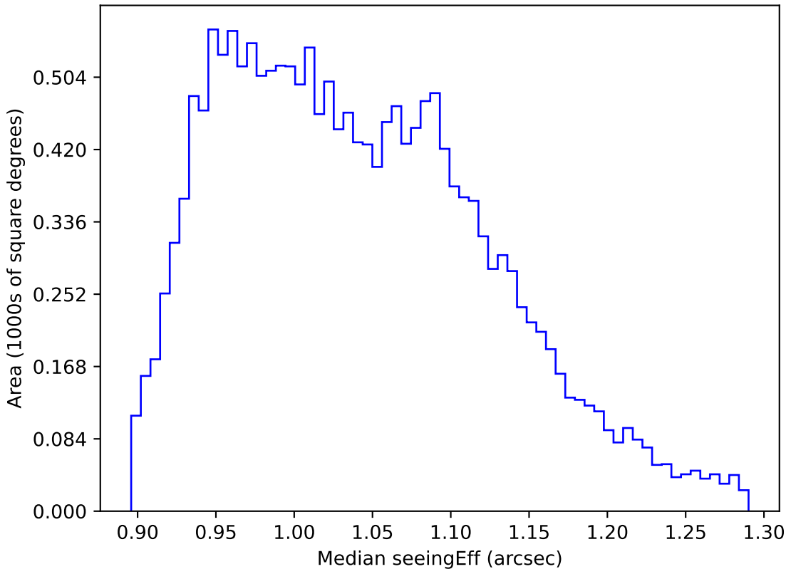
weather_cloudso6v3.4_10yrs WFD r band: Median seeingEff
