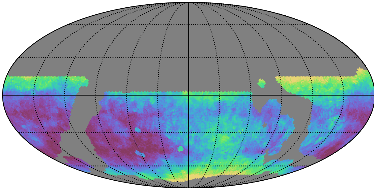
weather_cloudso6v3.4_10yrs WFD i band: Median seeingEff
