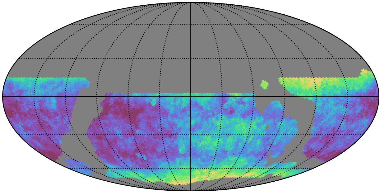
weather_cloudso6v3.4_10yrs WFD g band: Median seeingEff
