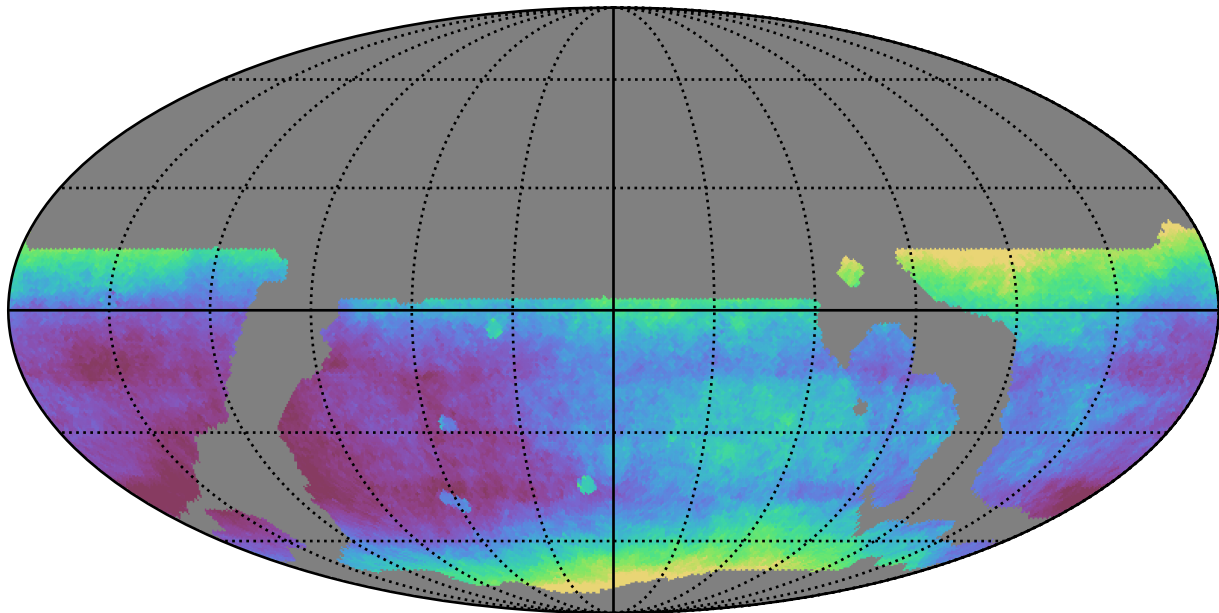
weather_cloudso6v3.4_10yrs WFD all bands: Median seeingEff
