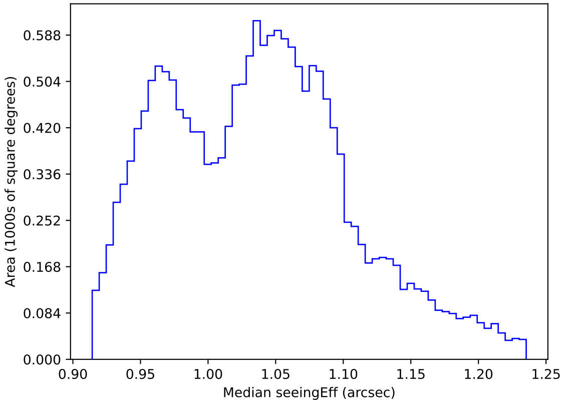
weather_cloudso6v3.4_10yrs WFD all bands: Median seeingEff
