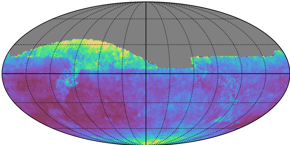
weather_cloudso6v3.4_10yrs All sky z band: Median seeingEff
