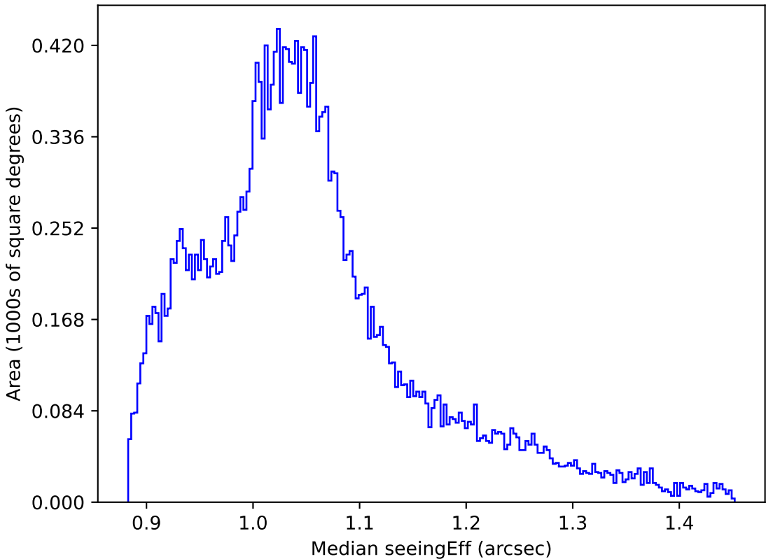
weather_cloudso6v3.4_10yrs All sky z band: Median seeingEff
