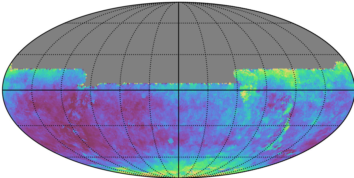
weather_cloudso6v3.4_10yrs All sky y band: Median seeingEff
