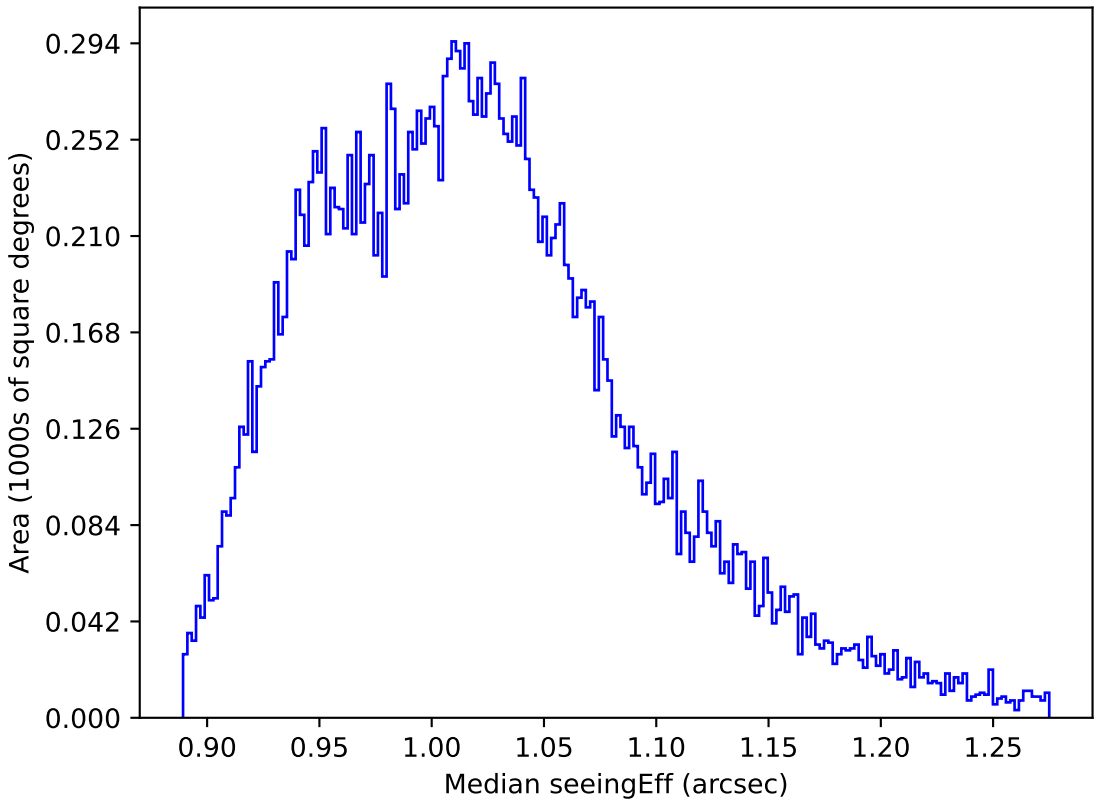
weather_cloudso6v3.4_10yrs All sky y band: Median seeingEff
