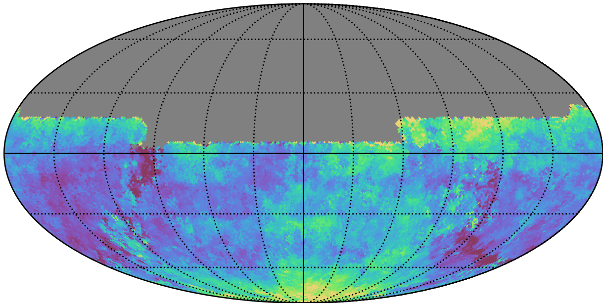
weather_cloudso6v3.4_10yrs All sky u band: Median seeingEff
