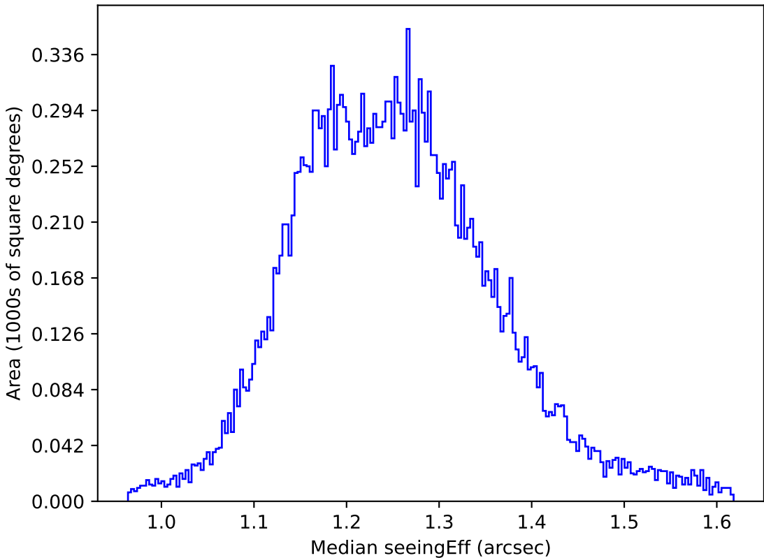
weather_cloudso6v3.4_10yrs All sky u band: Median seeingEff
