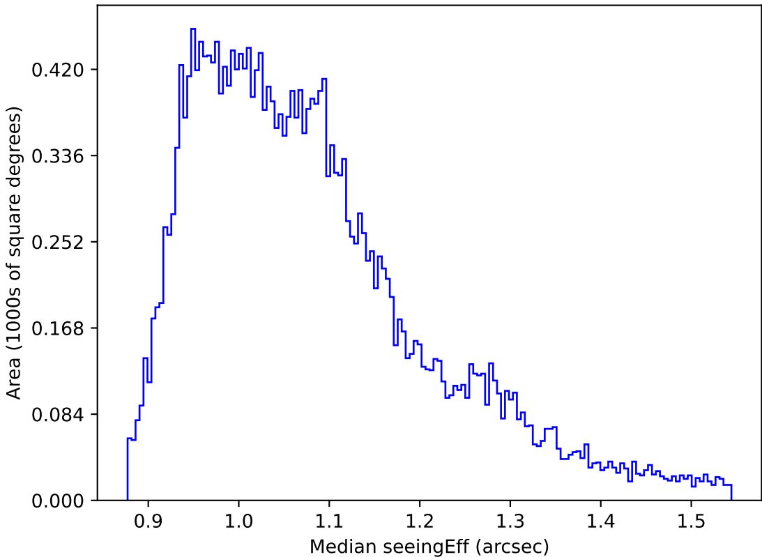
weather_cloudso6v3.4_10yrs All sky r band: Median seeingEff
