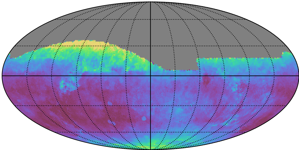
weather_cloudso6v3.4_10yrs All sky i band: Median seeingEff
