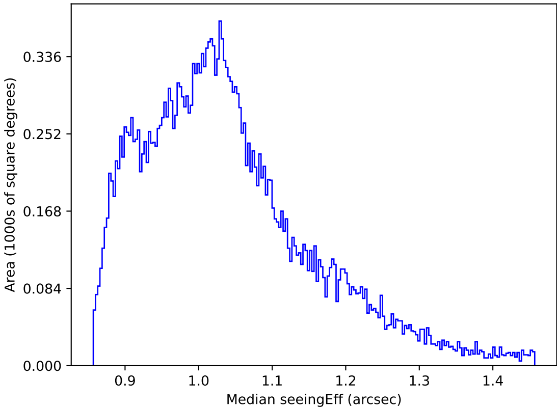
weather_cloudso6v3.4_10yrs All sky i band: Median seeingEff
