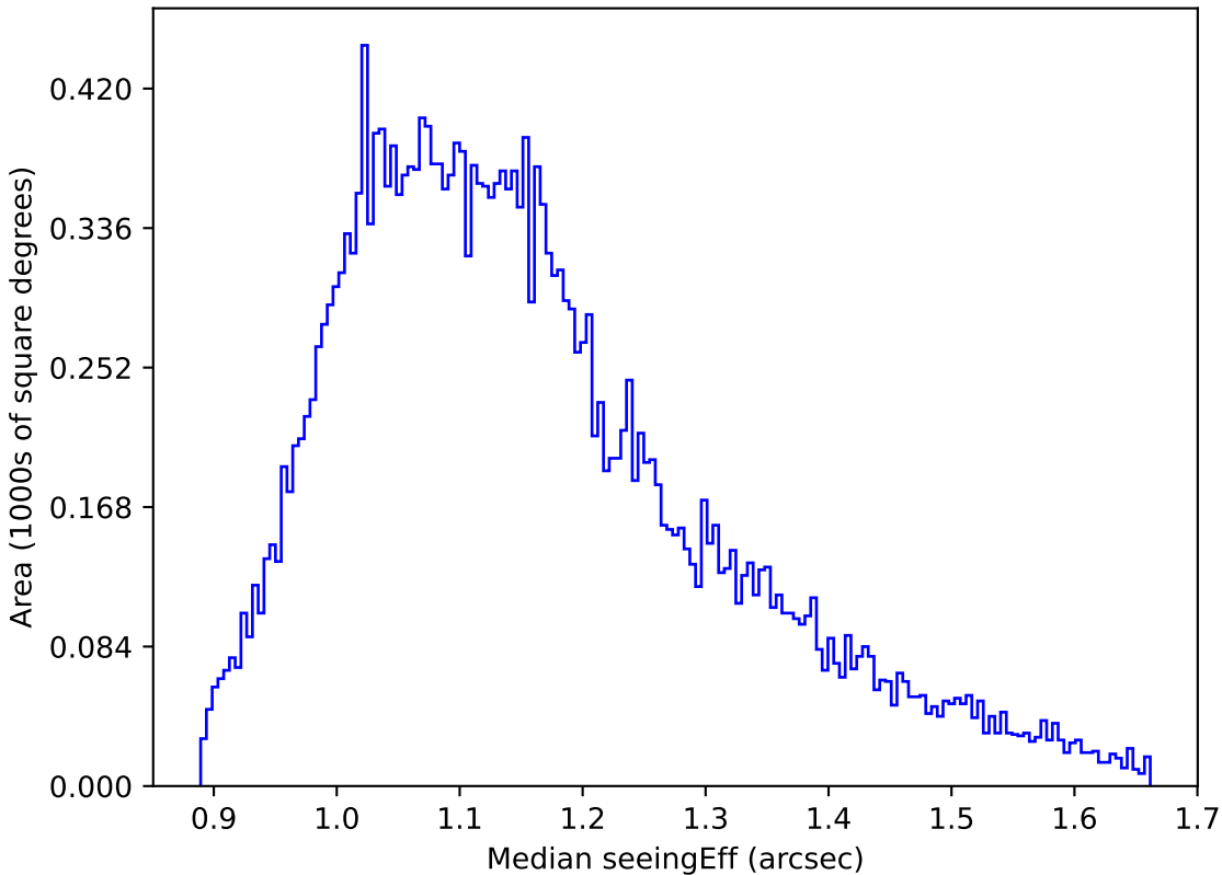
weather_cloudso6v3.4_10yrs All sky g band: Median seeingEff
