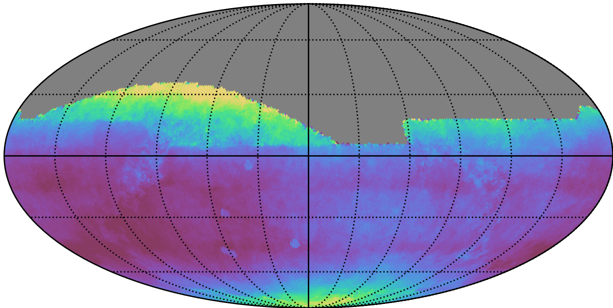
weather_cloudso6v3.4_10yrs All sky all bands: Median seeingEff
