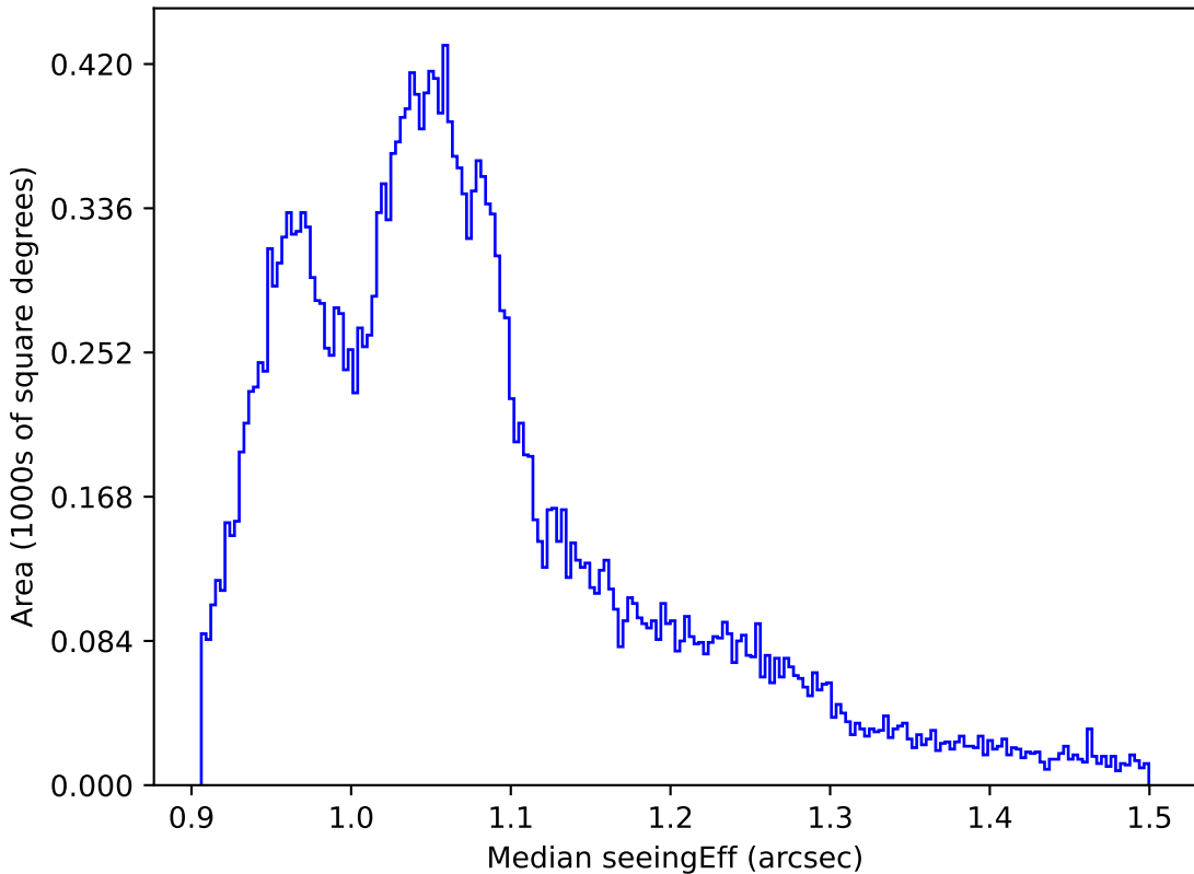
weather_cloudso6v3.4_10yrs All sky all bands: Median seeingEff
