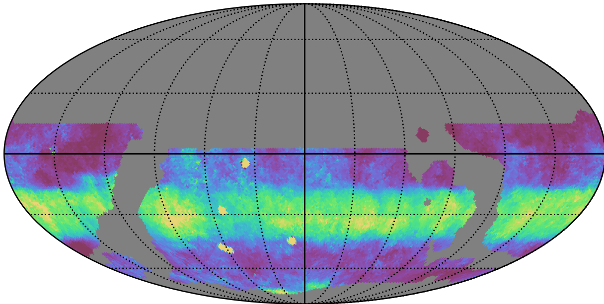
weather_cloudso6v3.4_10yrs WFD z band: Median normairmass
