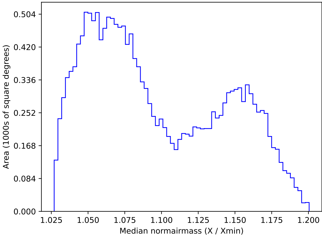
weather_cloudso6v3.4_10yrs WFD z band: Median normairmass
