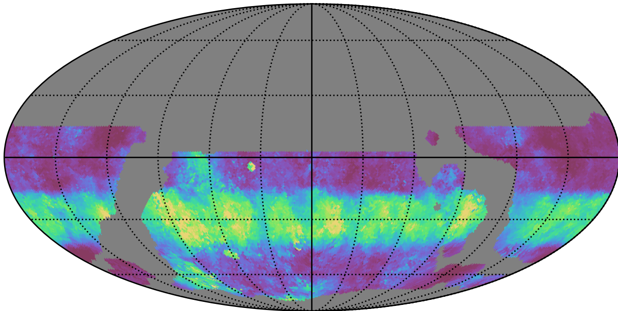
weather_cloudso6v3.4_10yrs WFD u band: Median normairmass
