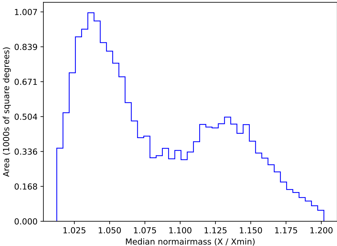
weather_cloudso6v3.4_10yrs WFD u band: Median normairmass
