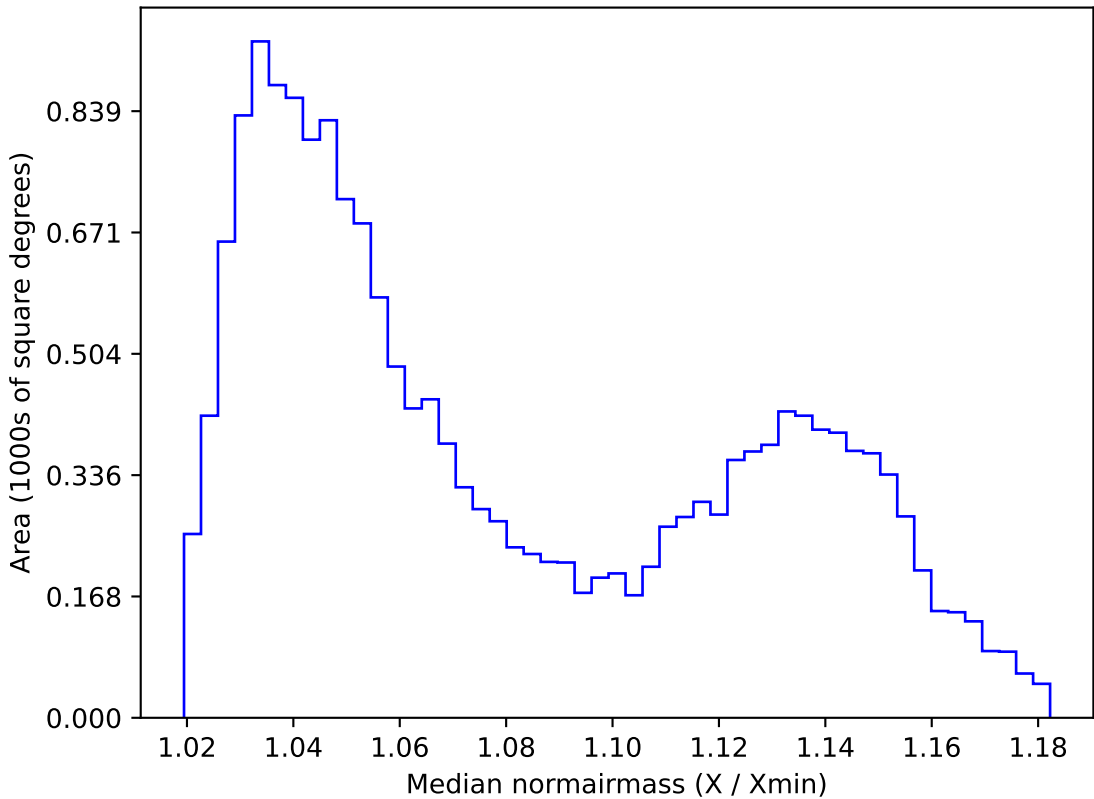
weather_cloudso6v3.4_10yrs WFD r band: Median normairmass
