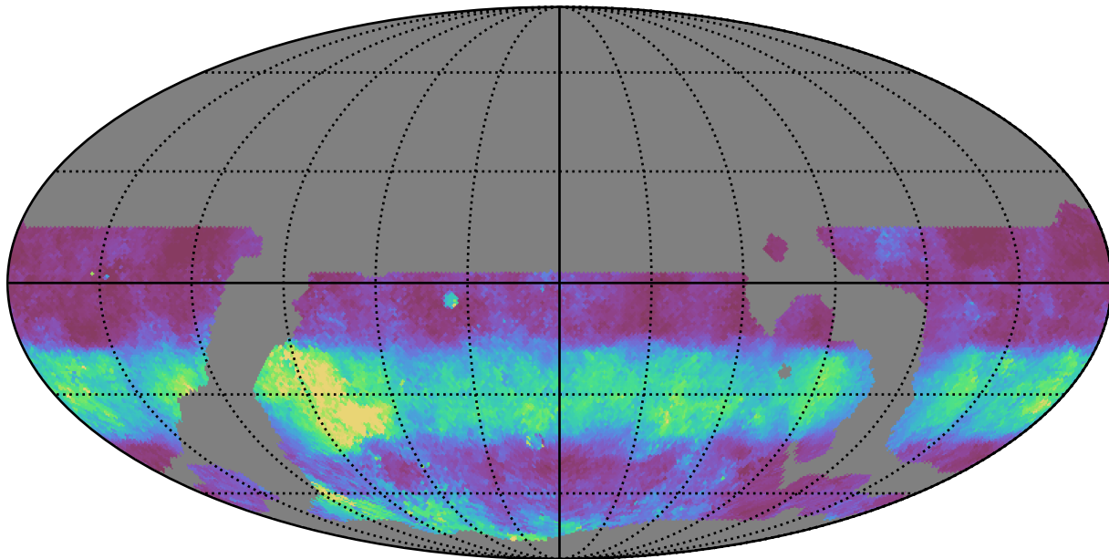
weather_cloudso6v3.4_10yrs WFD g band: Median normairmass
