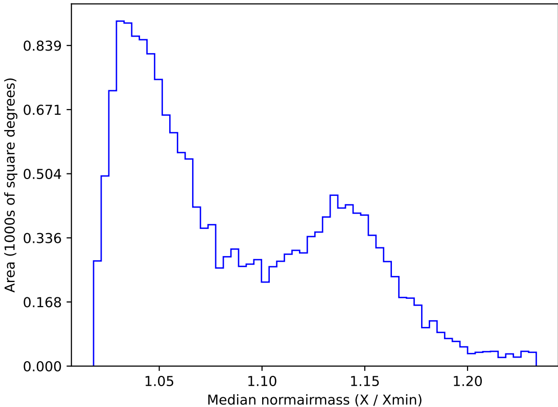
weather_cloudso6v3.4_10yrs WFD g band: Median normairmass
