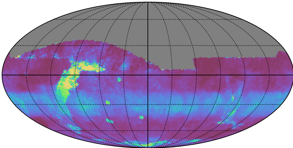
weather_cloudso6v3.4_10yrs All sky z band: Median normairmass
