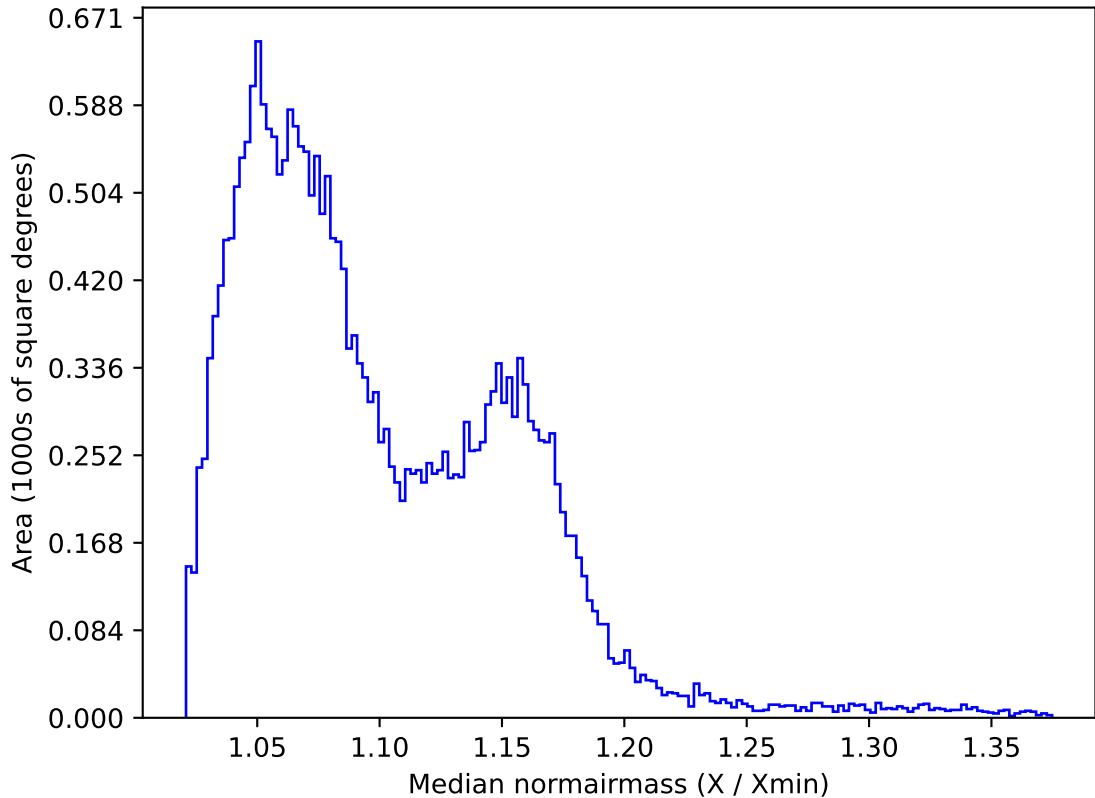
weather_cloudso6v3.4_10yrs All sky z band: Median normairmass
