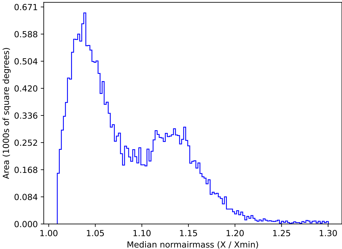
weather_cloudso6v3.4_10yrs All sky u band: Median normairmass
