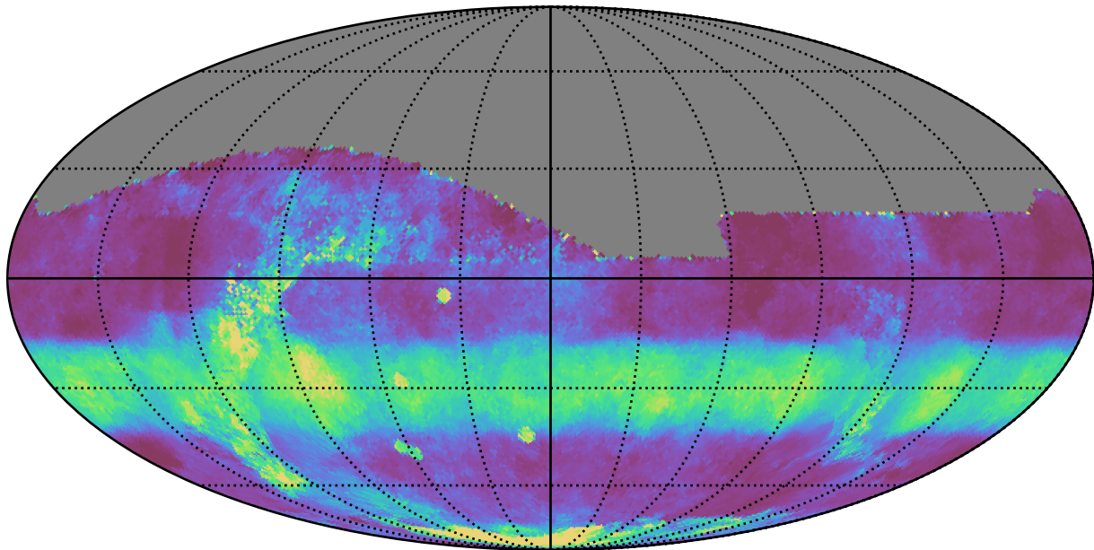
weather_cloudso6v3.4_10yrs All sky r band: Median normairmass
