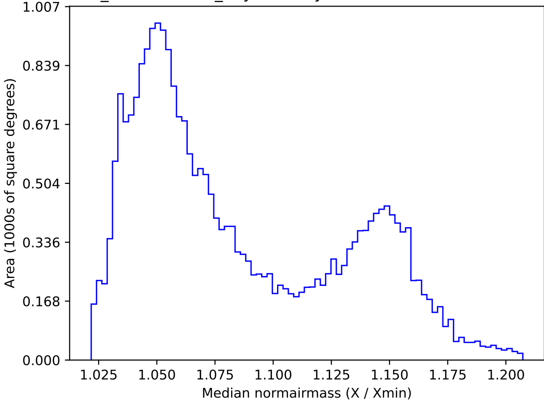
weather_cloudso6v3.4_10yrs All sky all bands: Median normairmass
