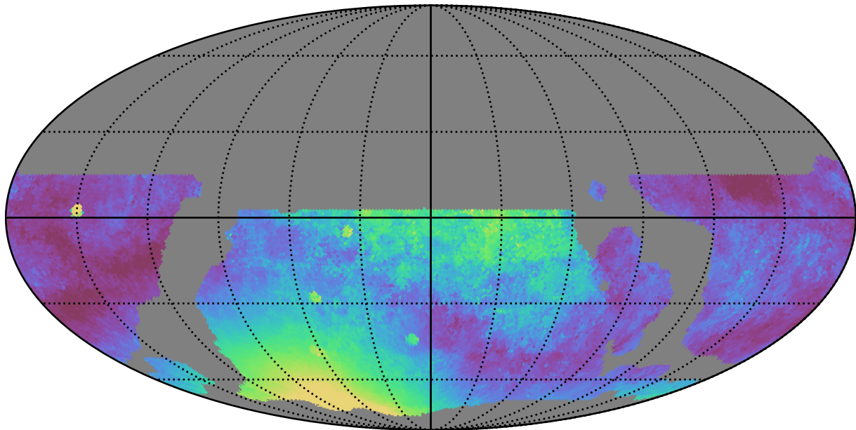
weather_cloudso6v3.4_10yrs WFD y band: Median moonDistance
